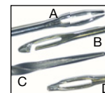
A=Split Eye C=Spiral Probe B=Open Eye D=Closed Eye
